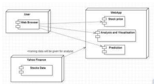
Fig 2: Proposed Architecture
